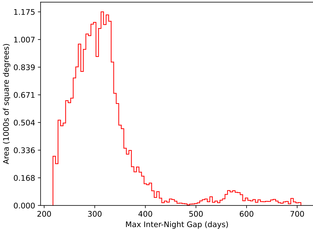
too_elab_r256_d2_griz_v3.4_10yrs All sky i band: Max Inter-Night Gap
