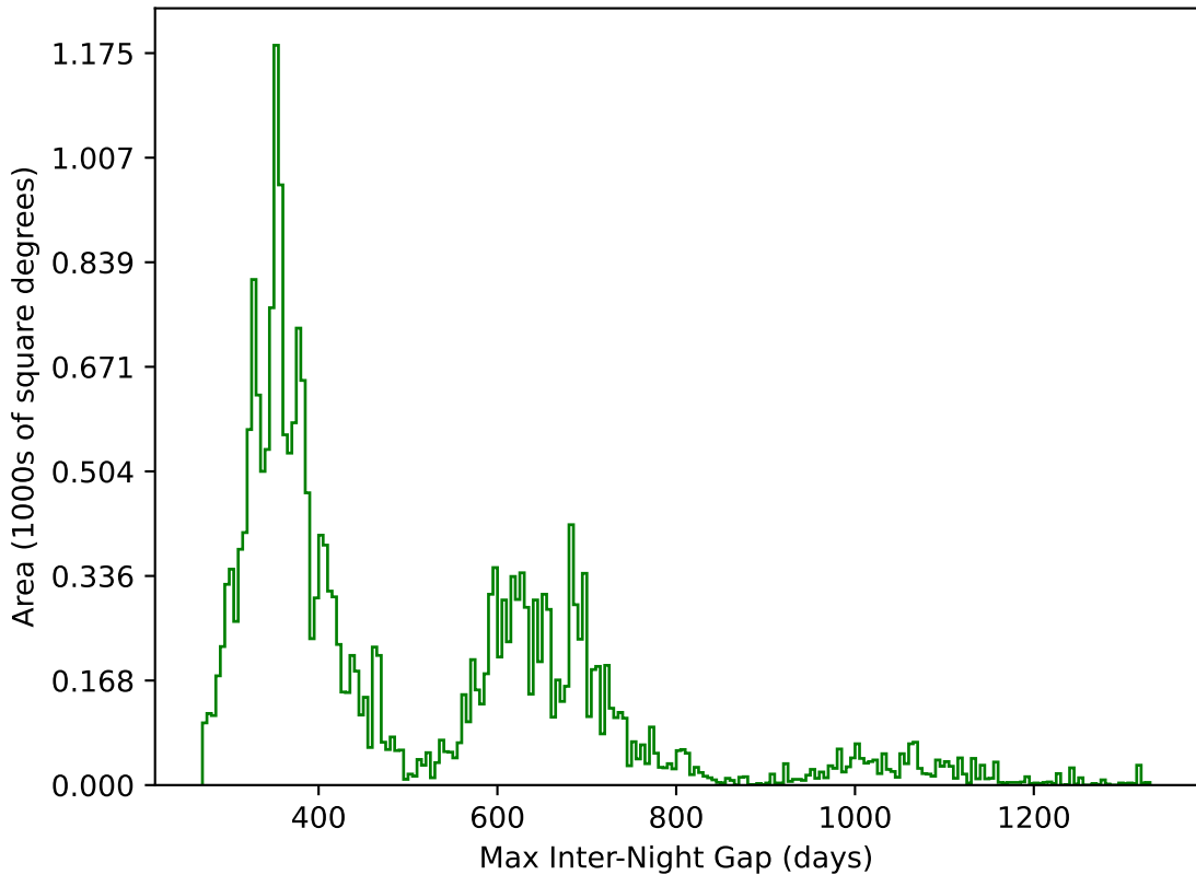
too_elab_r256_d2_griz_v3.4_10yrs All sky g band: Max Inter-Night Gap
