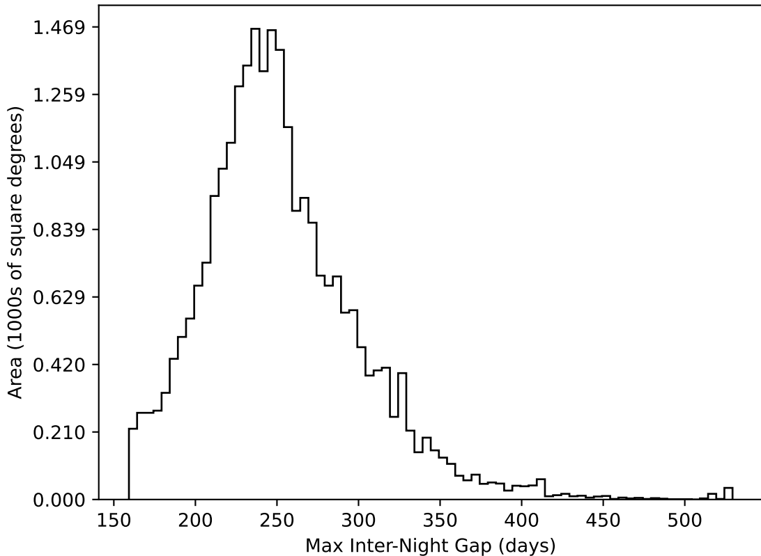
too_elab_r256_d2_griz_v3.4_10yrs All sky all bands: Max Inter-Night Gap
