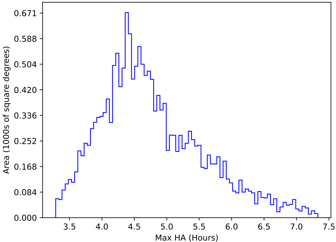
too_elab_r256_d2_griz_v3.4_10yrs WFD y band: Max HA
