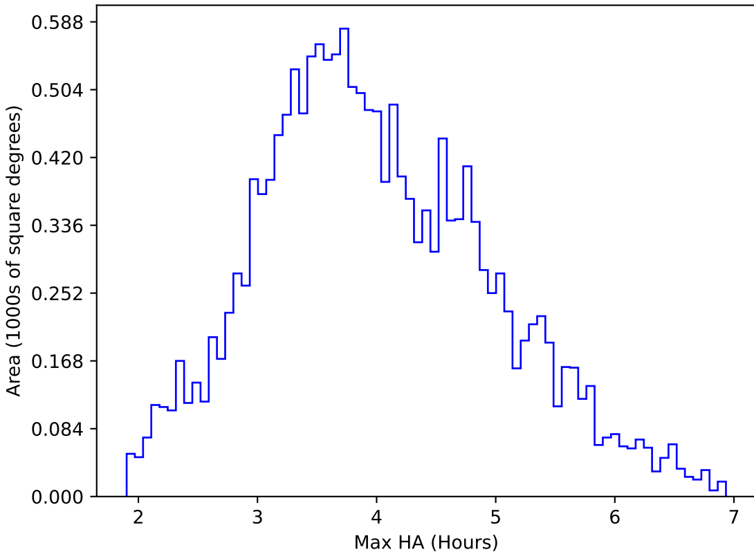
too_elab_r256_d2_griz_v3.4_10yrs WFD u band: Max HA
