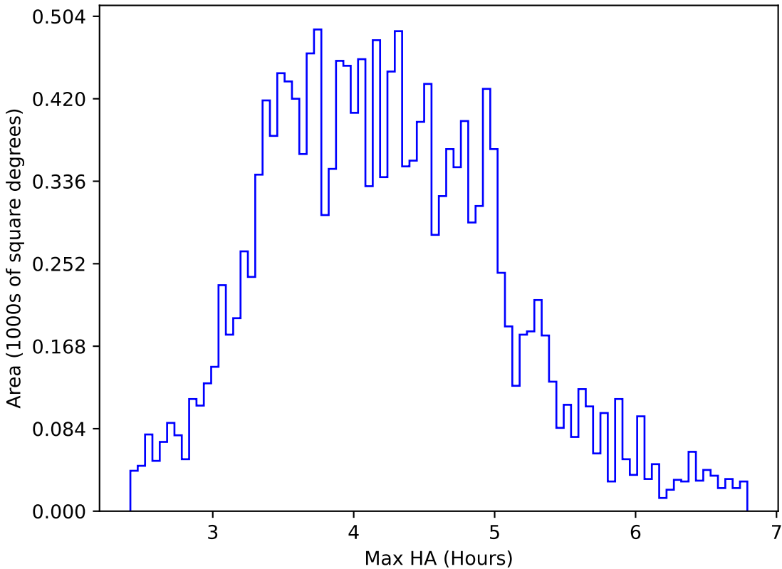
too_elab_r256_d2_griz_v3.4_10yrs WFD g band: Max HA
