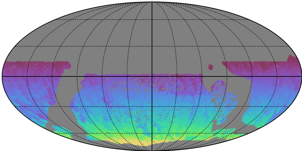
too_elab_r256_d2_griz_v3.4_10yrs WFD all bands: Max HA
