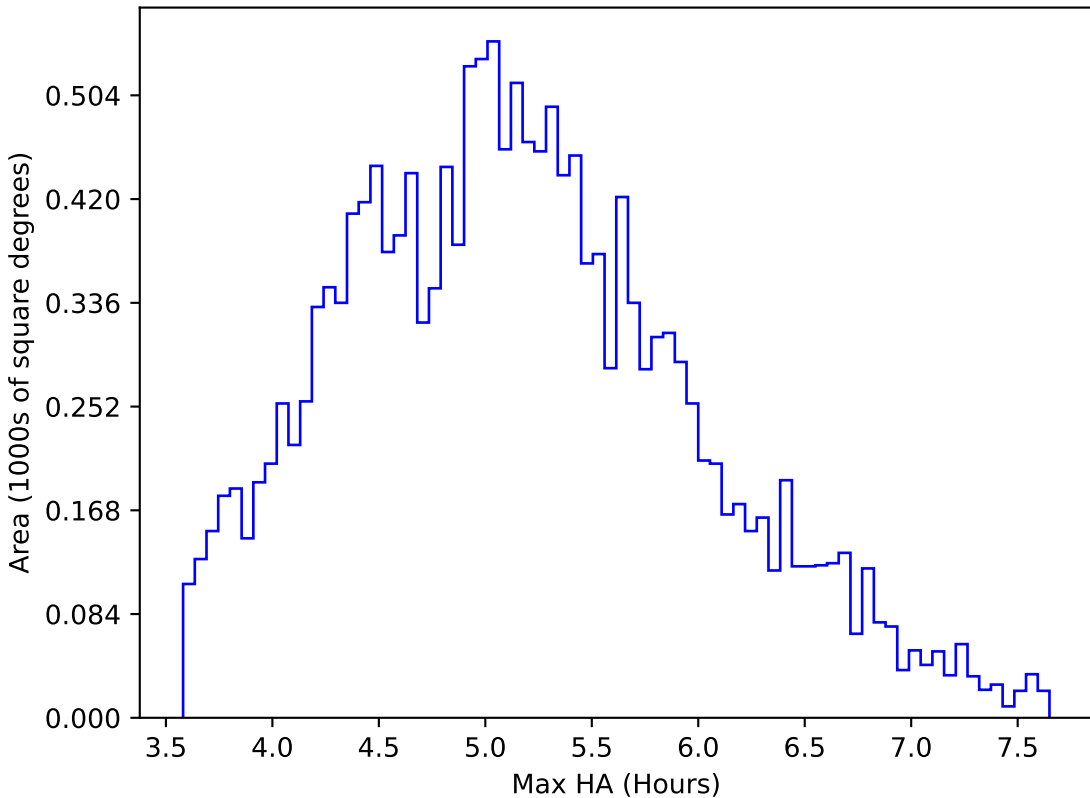
too_elab_r256_d2_griz_v3.4_10yrs WFD all bands: Max HA
