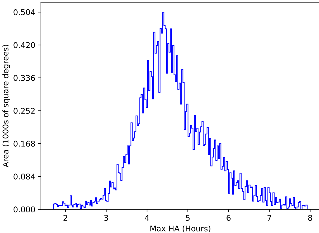
too_elab_r256_d2_griz_v3.4_10yrs All sky y band: Max HA
