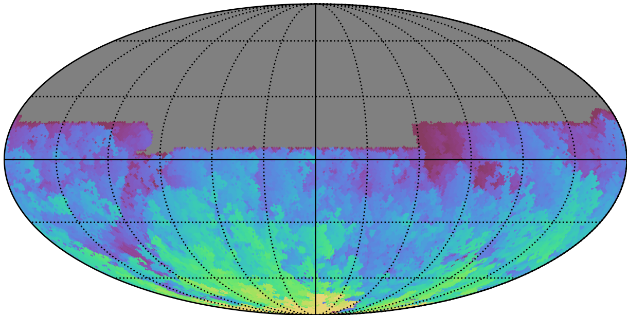
too_elab_r256_d2_griz_v3.4_10yrs All sky u band: Max HA
