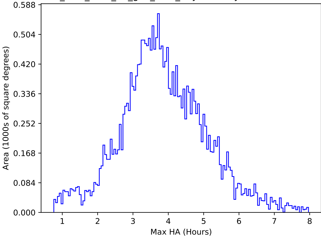
too_elab_r256_d2_griz_v3.4_10yrs All sky u band: Max HA
