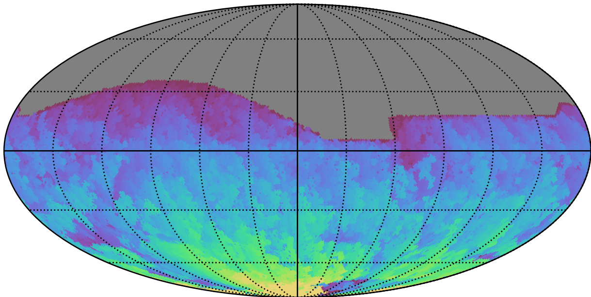
too_elab_r256_d2_griz_v3.4_10yrs All sky r band: Max HA
