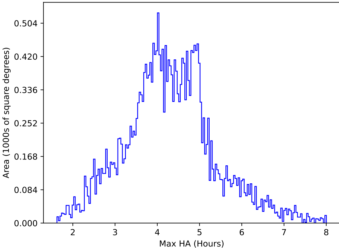
too_elab_r256_d2_griz_v3.4_10yrs All sky r band: Max HA
