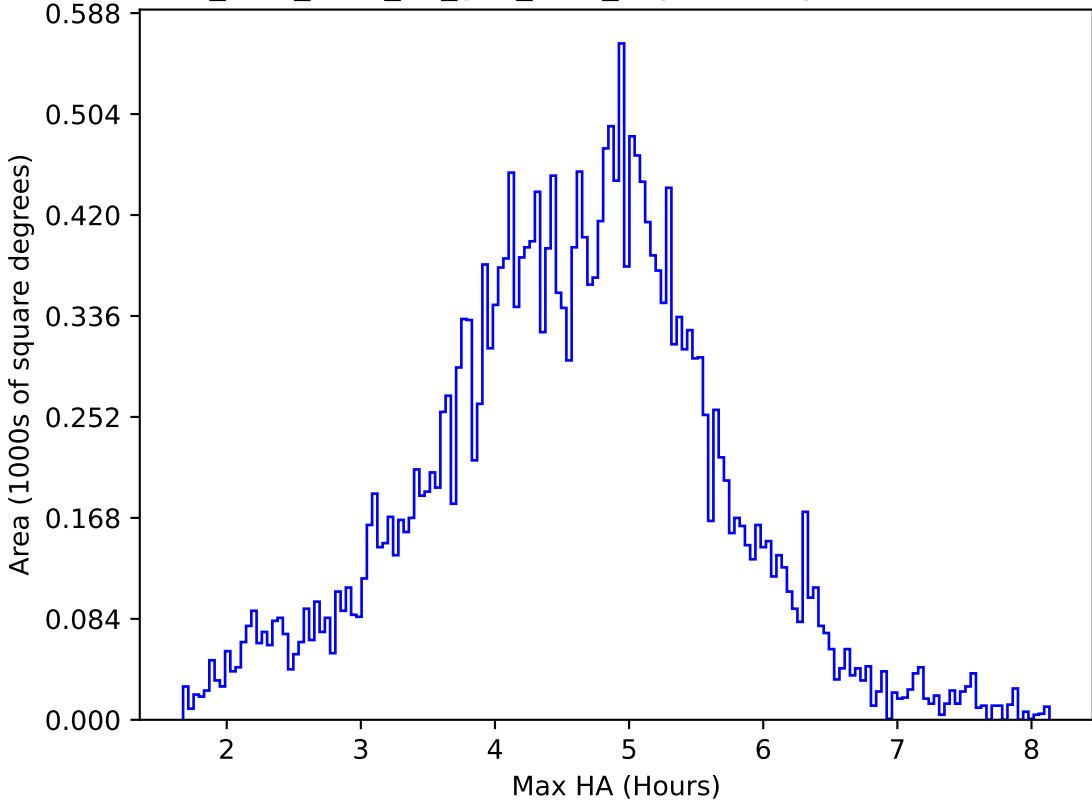
too_elab_r256_d2_griz_v3.4_10yrs All sky i band: Max HA
