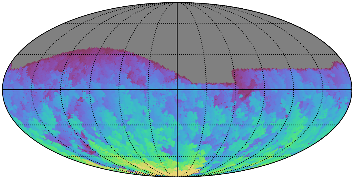
too_elab_r256_d2_griz_v3.4_10yrs All sky g band: Max HA
