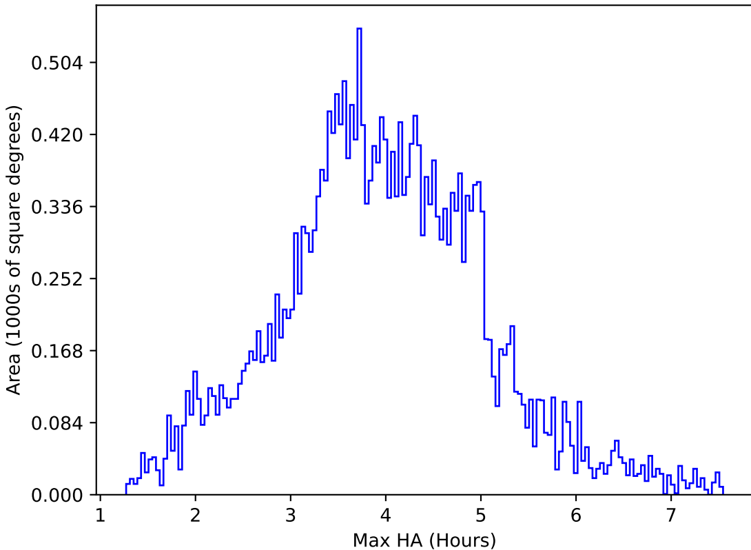
too_elab_r256_d2_griz_v3.4_10yrs All sky g band: Max HA
