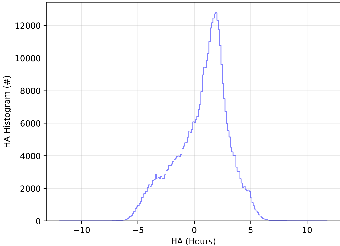
too_elab_r256_d2_griz_v3.4_10yrs WFD z band: HA Histogram
