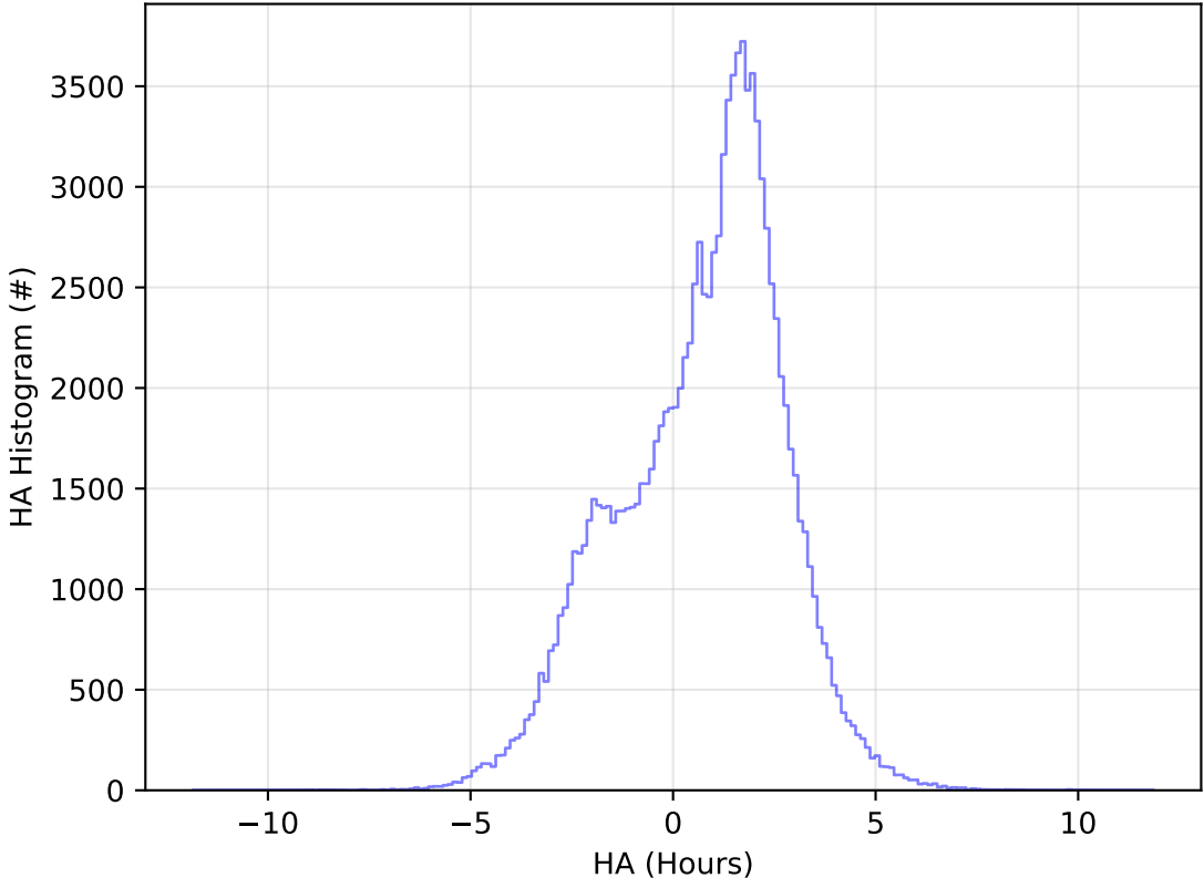
too_elab_r256_d2_griz_v3.4_10yrs WFD u band: HA Histogram
