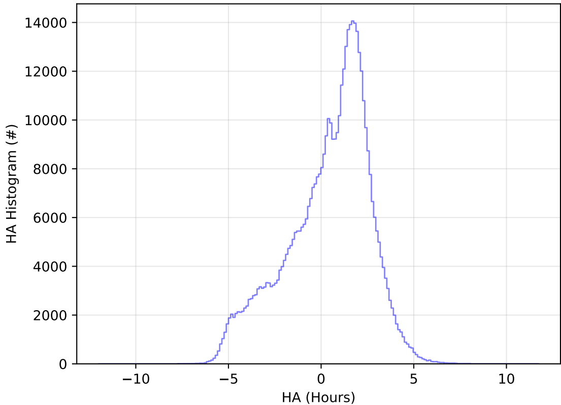
too_elab_r256_d2_griz_v3.4_10yrs WFD r band: HA Histogram
