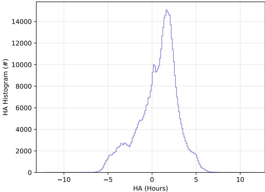
too_elab_r256_d2_griz_v3.4_10yrs WFD i band: HA Histogram
