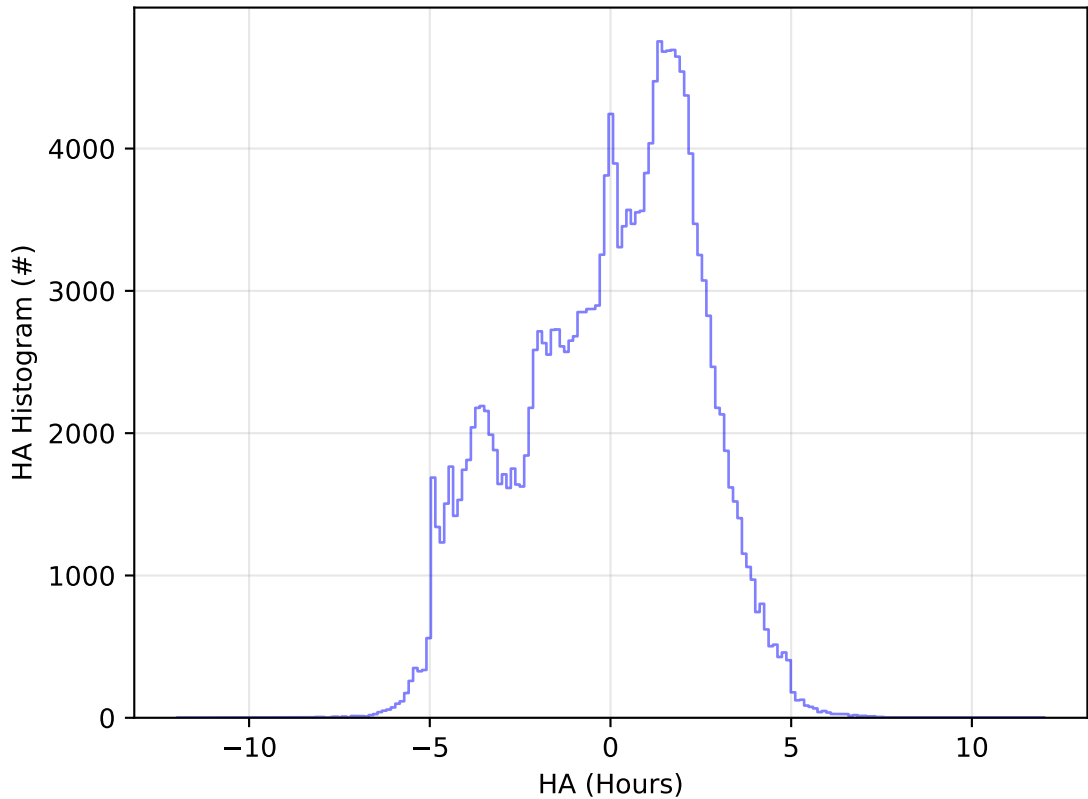
too_elab_r256_d2_griz_v3.4_10yrs WFD g band: HA Histogram
