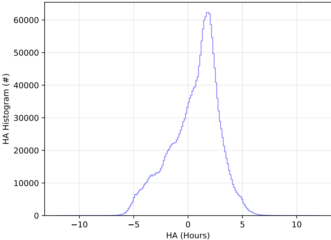
too_elab_r256_d2_griz_v3.4_10yrs WFD all bands: HA Histogram
