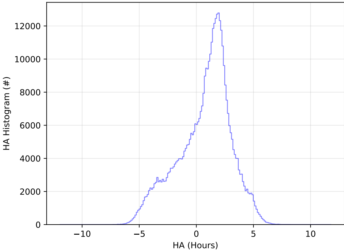
too_elab_r256_d2_griz_v3.4_10yrs All sky z band: HA Histogram
