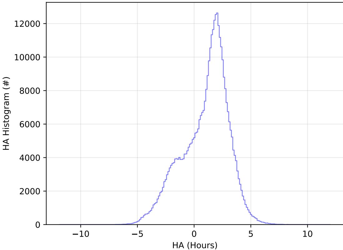
too_elab_r256_d2_griz_v3.4_10yrs All sky y band: HA Histogram
