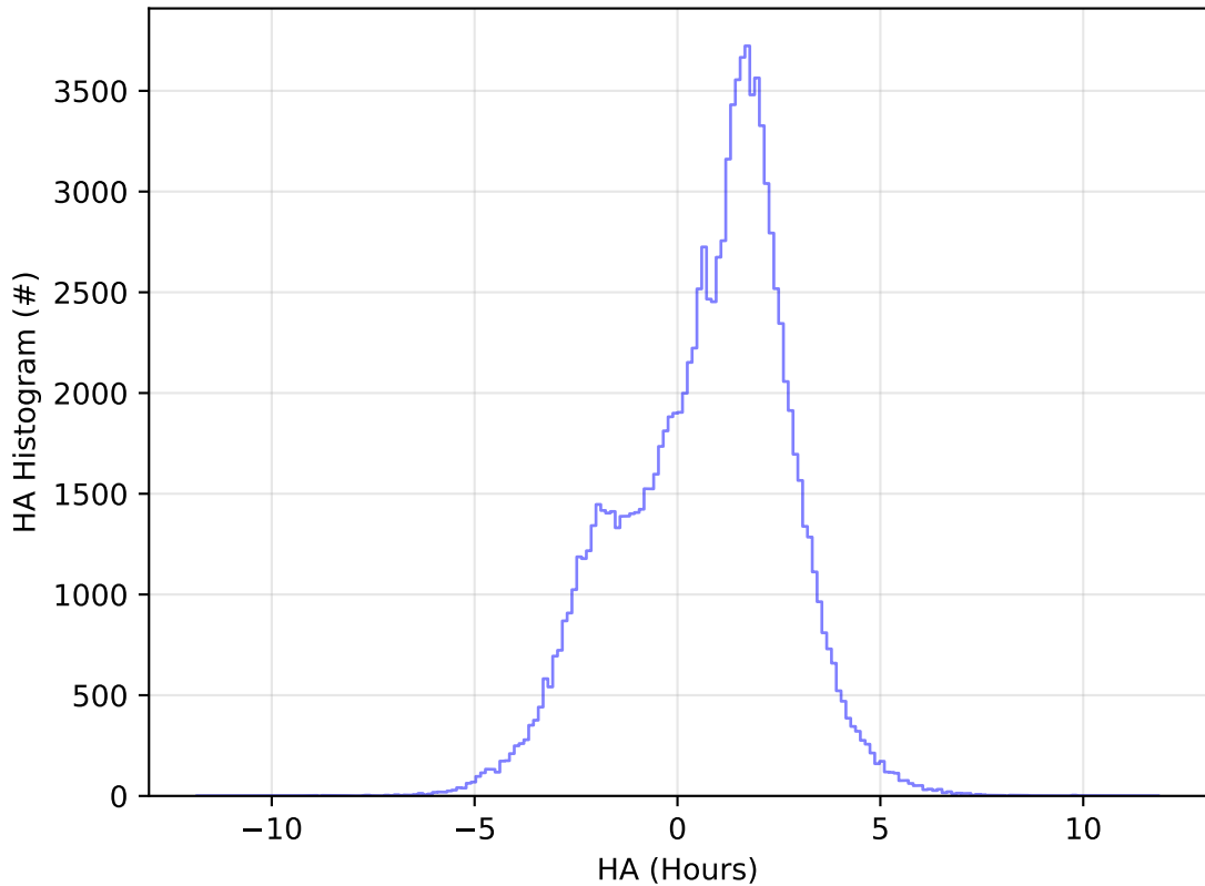
too_elab_r256_d2_griz_v3.4_10yrs All sky u band: HA Histogram
