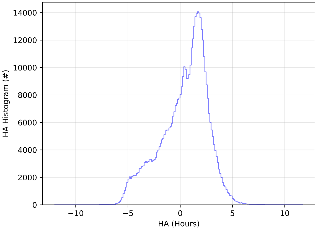
too_elab_r256_d2_griz_v3.4_10yrs All sky r band: HA Histogram
