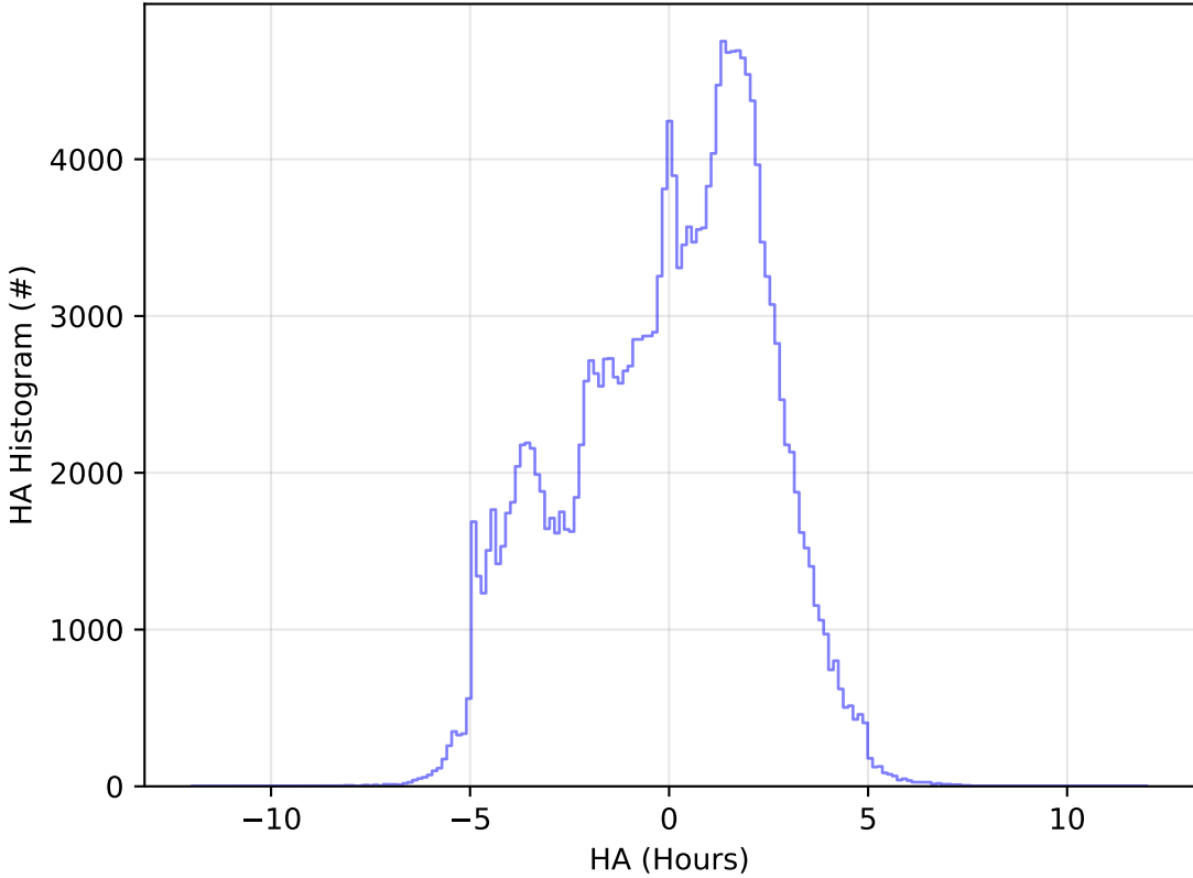
too_elab_r256_d2_griz_v3.4_10yrs All sky g band: HA Histogram
