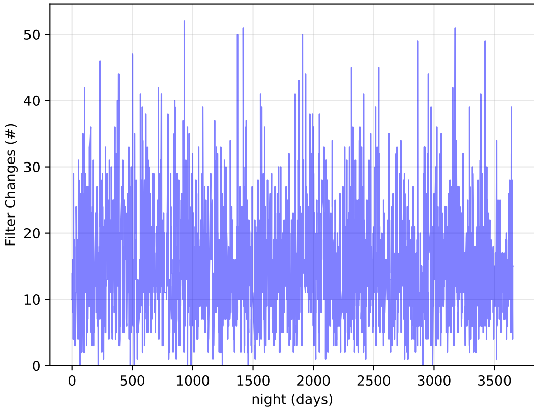
too_elab_r256_d2_griz_v3.4_10yrs Per Night: Filter Changes
