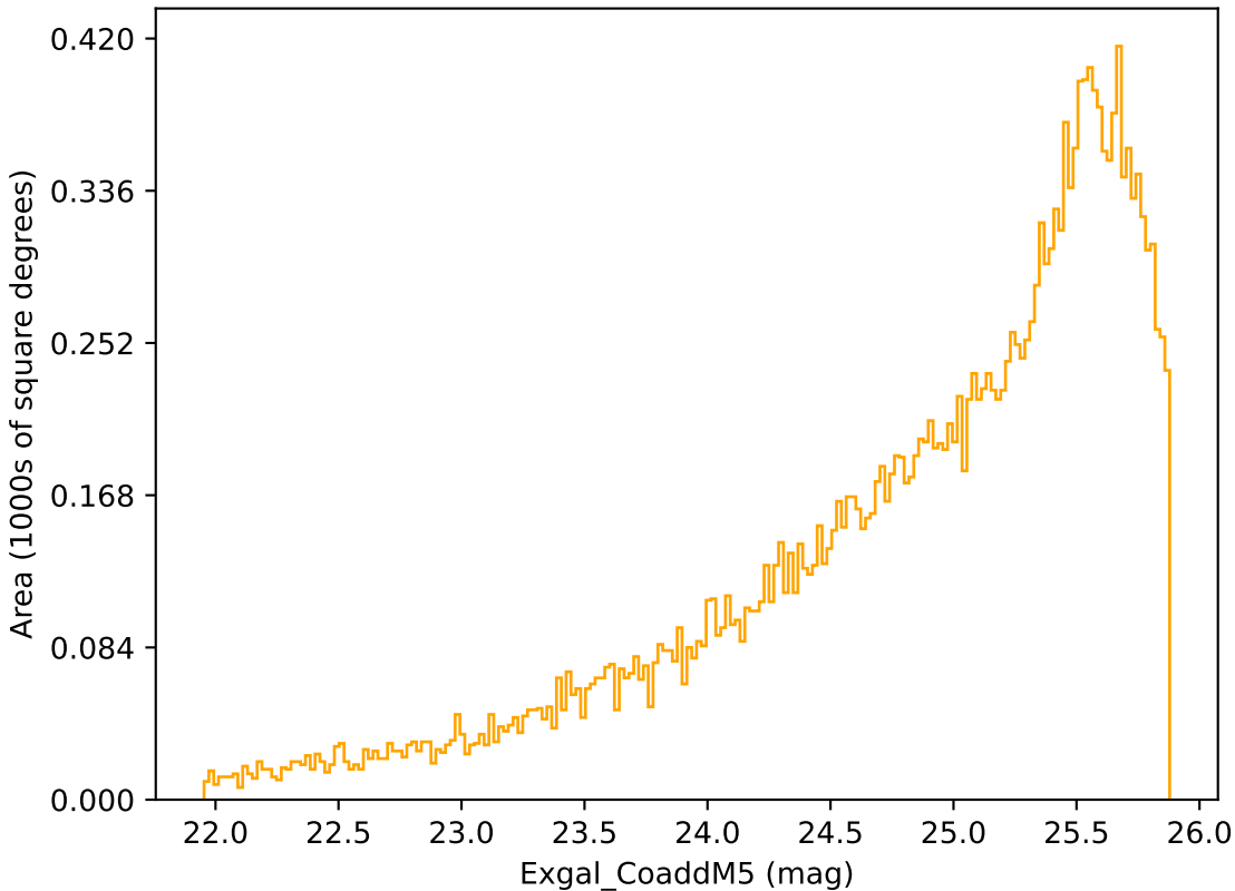
too_elab_r256_d2_griz_v3.4_10yrs Yr 3-4 r band: Exgal_CoaddM5
