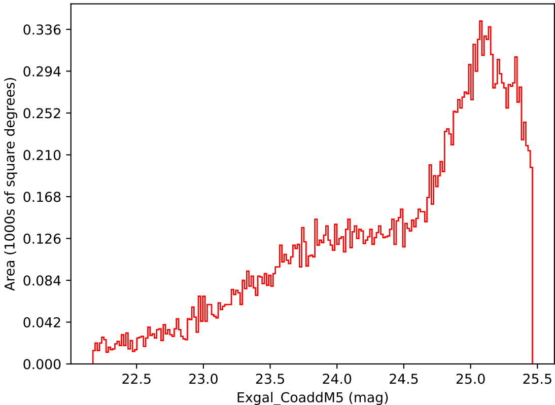
too_elab_r256_d2_griz_v3.4_10yrs Yr 3-4 i band: Exgal_CoaddM5
