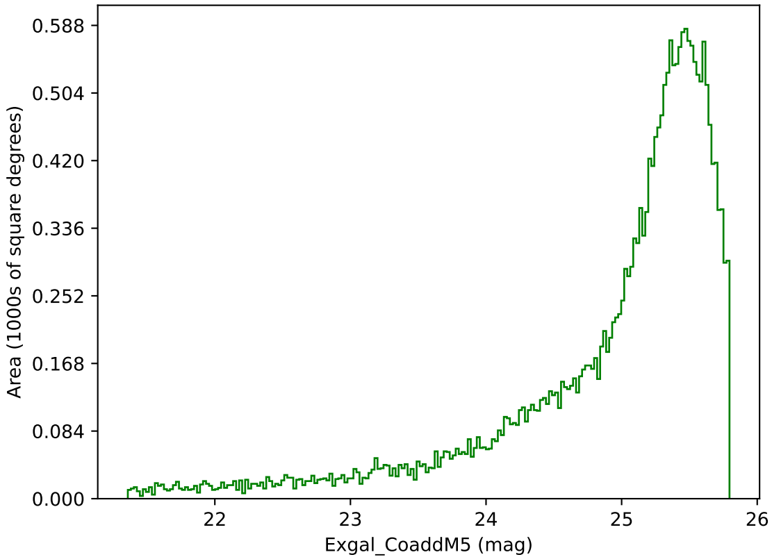
too_elab_r256_d2_griz_v3.4_10yrs Yr 1 g band: Exgal_CoaddM5
