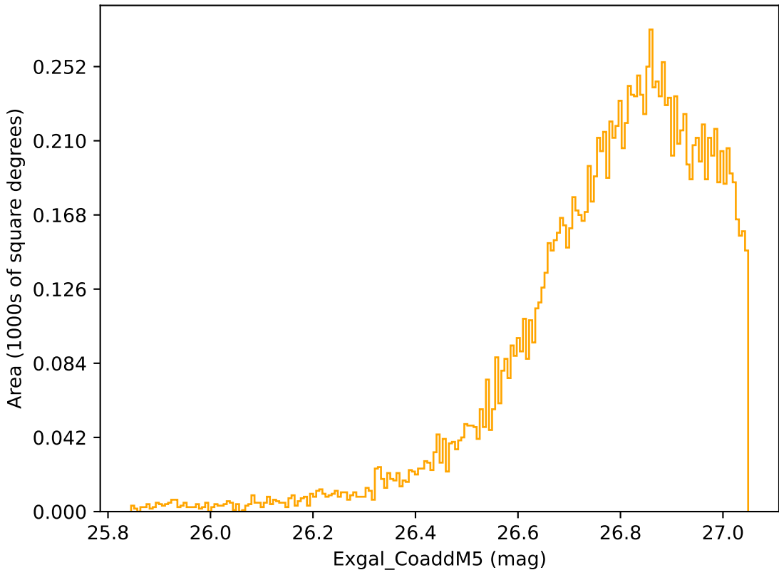
too_elab_r256_d2_griz_v3.4_10yrs WFD r band: Exgal_CoaddM5
