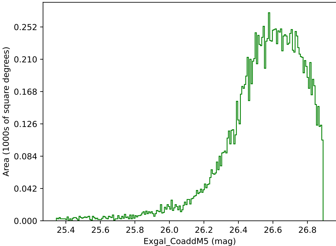
too_elab_r256_d2_griz_v3.4_10yrs WFD g band: Exgal_CoaddM5
