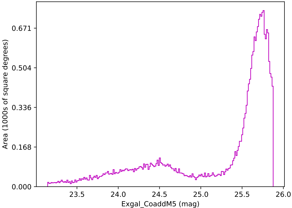
too_elab_r256_d2_griz_v3.4_10yrs All sky z band: Exgal_CoaddM5
