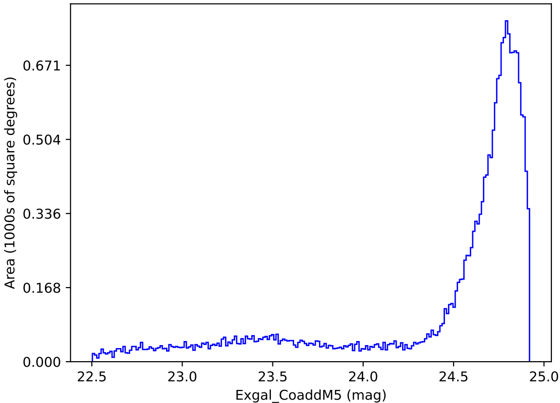
too_elab_r256_d2_griz_v3.4_10yrs All sky y band: Exgal_CoaddM5
