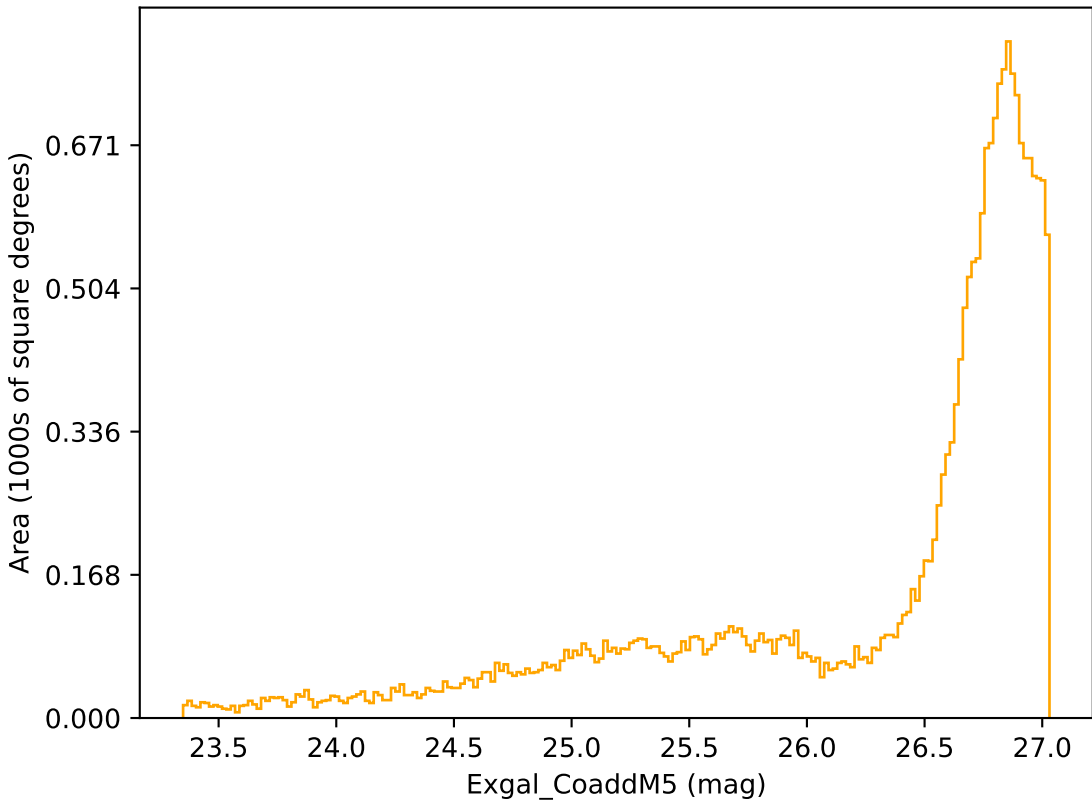
too_elab_r256_d2_griz_v3.4_10yrs All sky r band: Exgal_CoaddM5
