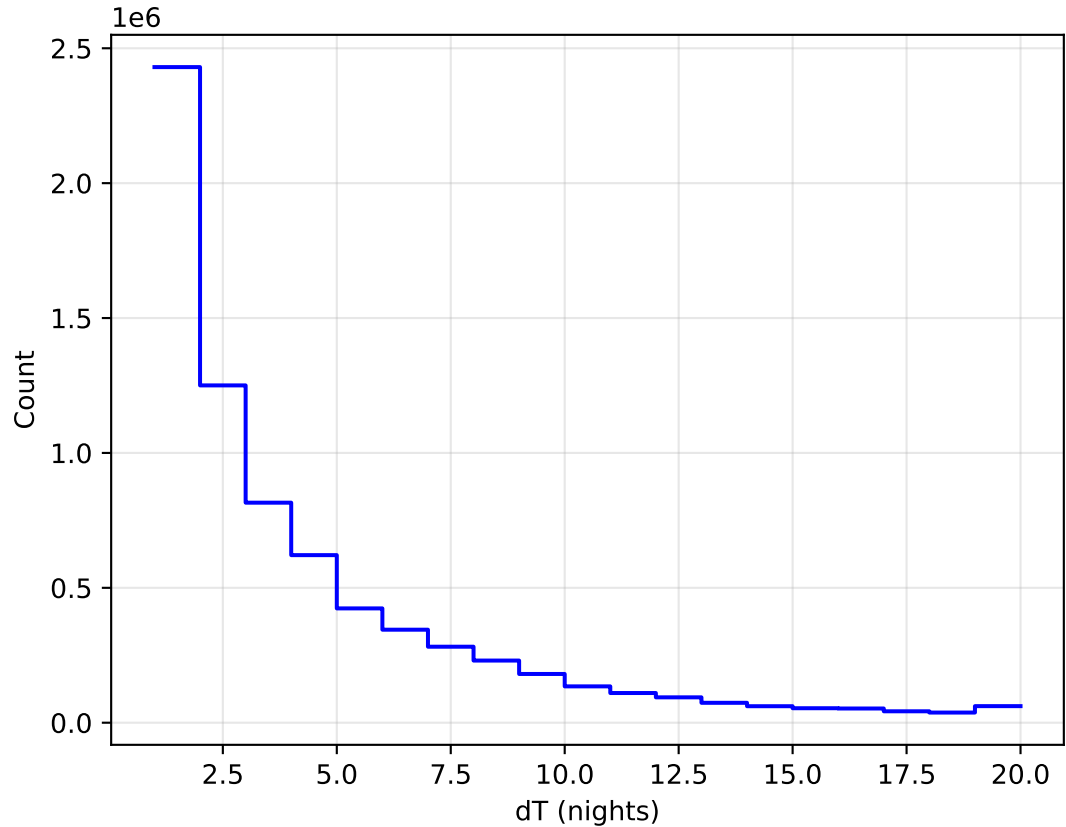
too_elab_r256_d2_griz_v3.4_10yrs WFD all bands: DeltaNight Histogram
