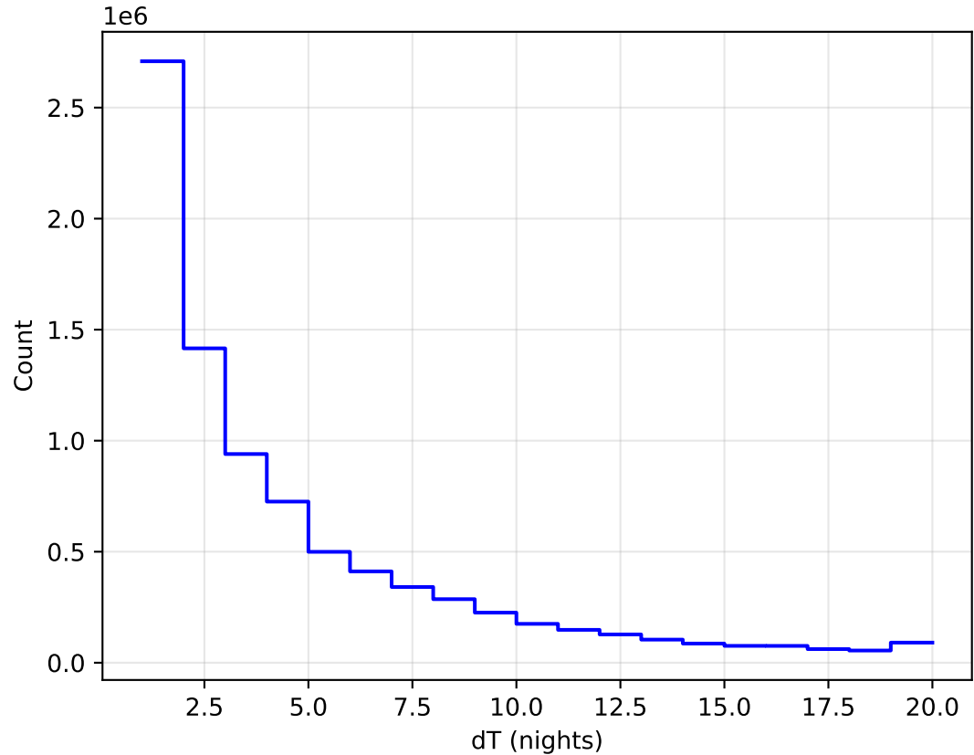
too_elab_r256_d2_griz_v3.4_10yrs All sky all bands: DeltaNight Histogram
