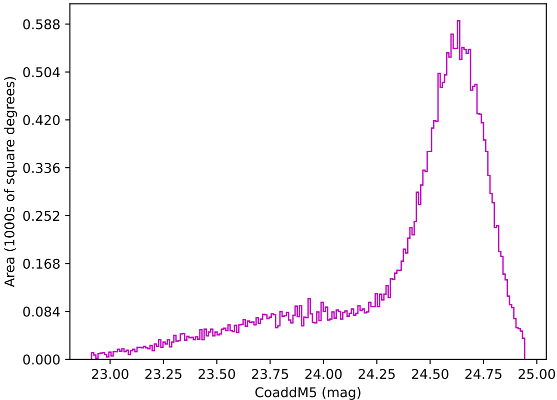
too_elab_r256_d2_griz_v3.4_10yrs Yr 1 z band: CoaddM5
