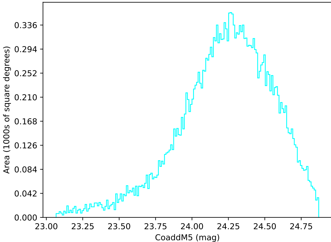
too_elab_r256_d2_griz_v3.4_10yrs Yr 1 u band: CoaddM5
