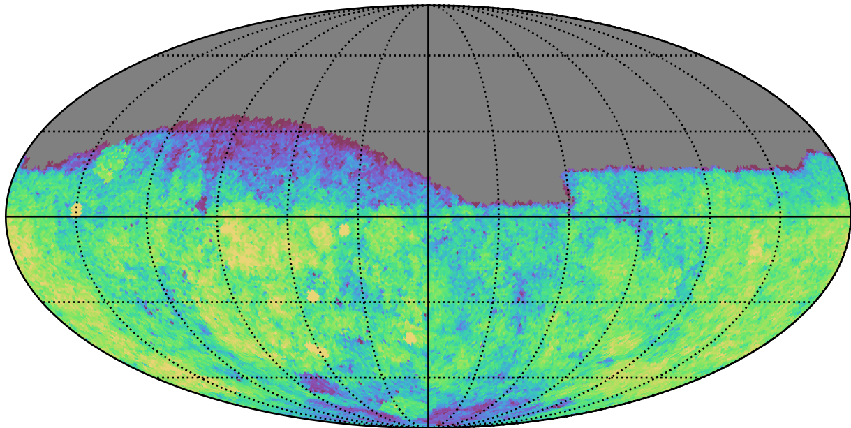
too_elab_r256_d2_griz_v3.4_10yrs Yr 1 g band: CoaddM5
