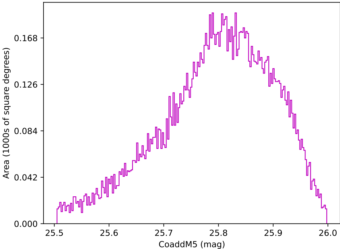
too_elab_r256_d2_griz_v3.4_10yrs WFD z band: CoaddM5
