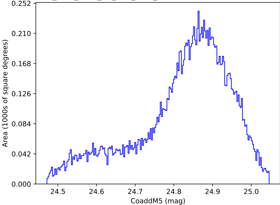
too_elab_r256_d2_griz_v3.4_10yrs WFD y band: CoaddM5
