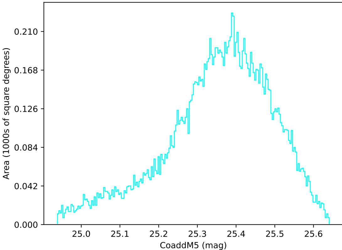
too_elab_r256_d2_griz_v3.4_10yrs WFD u band: CoaddM5
