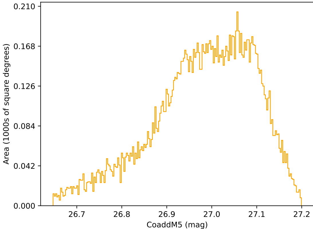
too_elab_r256_d2_griz_v3.4_10yrs WFD r band: CoaddM5
