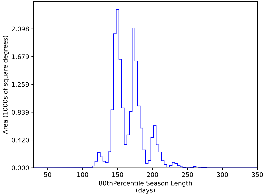
too_elab_r256_d2_griz_v3.4_10yrs WFD y band: 80thPercentile Season Length
