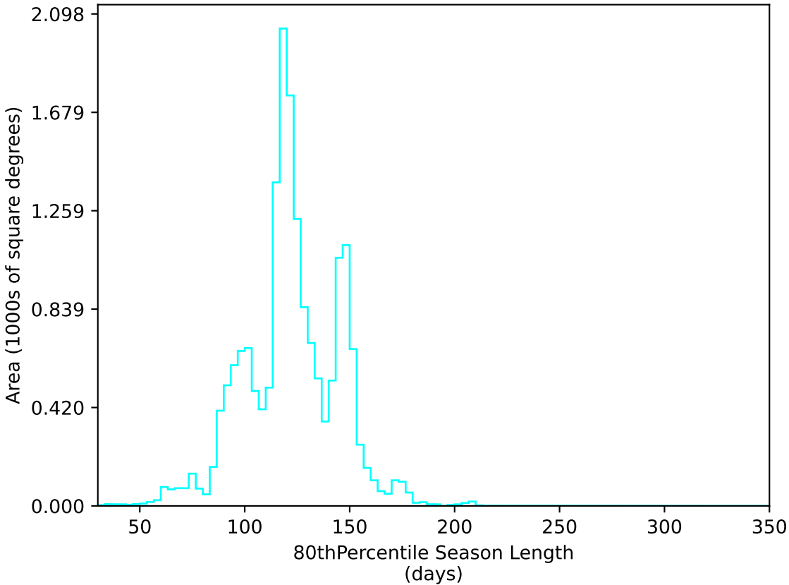
too_elab_r256_d2_griz_v3.4_10yrs WFD u band: 80thPercentile Season Length
