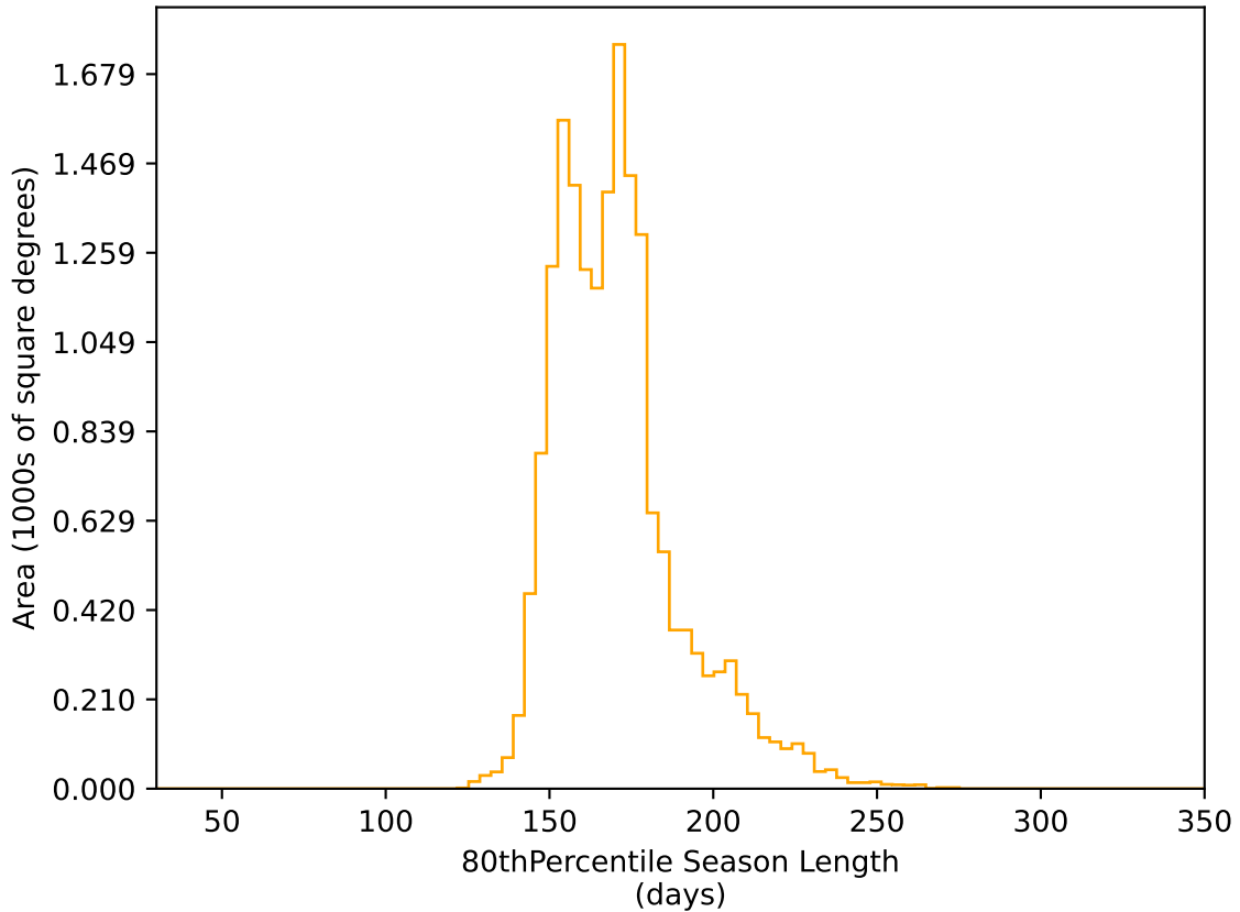
too_elab_r256_d2_griz_v3.4_10yrs WFD r band: 80thPercentile Season Length
