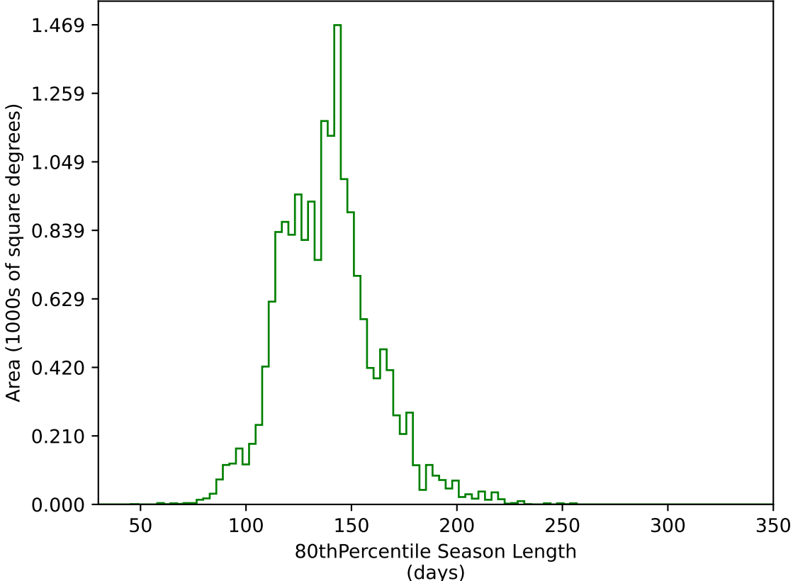
too_elab_r256_d2_griz_v3.4_10yrs WFD g band: 80thPercentile Season Length
