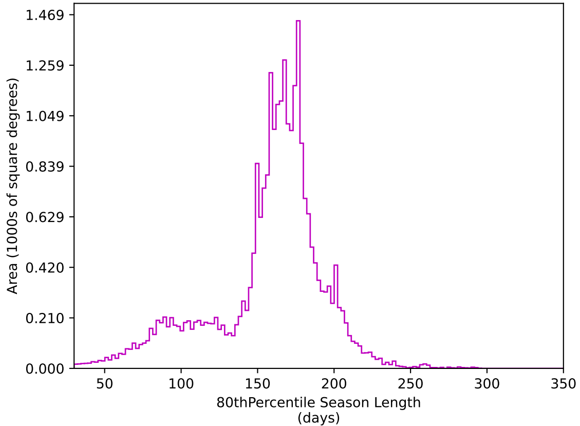
too_elab_r256_d2_griz_v3.4_10yrs All sky z band: 80thPercentile Season Length
